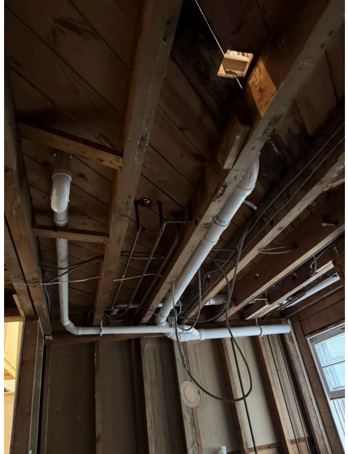
In progress: new PVC drain lines
